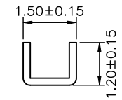
SEC:C-C
