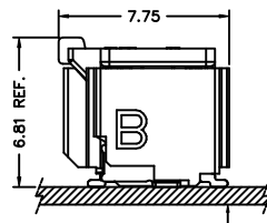
MATED CONDITION PCB
